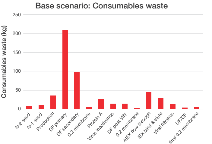
Figure 5: Consumable usage per process step
