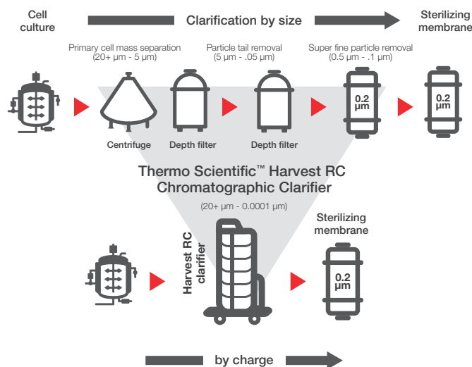
Figure 1: Thermo Scientific™ Harvest RC Chromatographic Clarifier reduces the harvest and clarification to a single stage unit operation.
