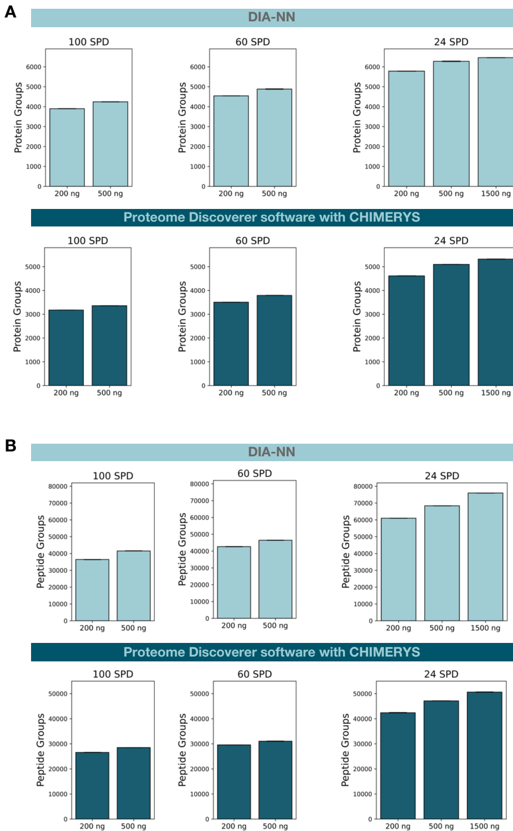
Figure 4. The Orbitrap Astral mass spectrometer coupled with the Seer Proteograph XT Assay enables deep plasma proteome coverage. The number of protein groups (A) and peptide groups (B) identified from different loads of enriched plasma. Samples were analyzed on the Orbitrap Astral mass spectrometer with 100 and 60 SPD high-throughput methods or a 24 SPD method to maximize identification.
