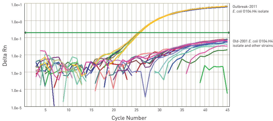
Figure 6. Identification of virulent strain in foods without false positives from closely related strains. Newly designed Custom TaqMan® E. coli O104:H4 (2011 Outbreak) Assay effectively detects the E. coli O104:H4 isolate responsible for the 2011 German E. coli outbreak and does not detect other closely related STEC strains.
